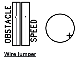
Wire jumper
